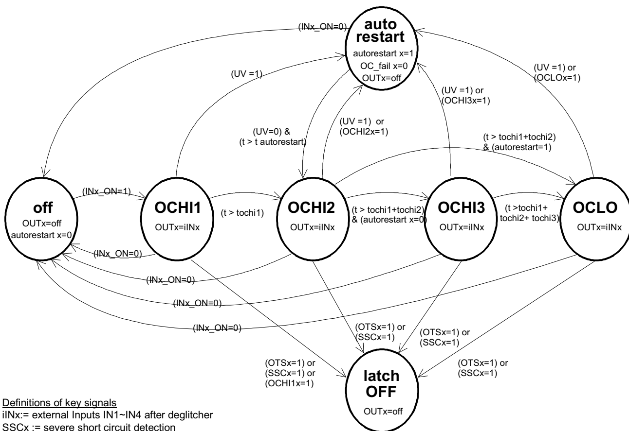
Figure 13. Output control diagram in fail mode
